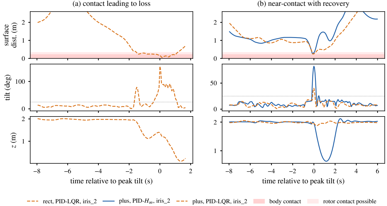
FIGURE 6. Upset events, aligned at peak tilt. Top: centre-to-surface distance to the nearest static cylinder (dark band: body contact, light band: rotor contact possible); middle: tilt (dotted: 25^\circ level-out threshold); bottom: altitude. (a) PID-LQR, rect, agent 2: contact and loss. (b) plus , agent 2 under both controllers: grazing contact and recovery.
